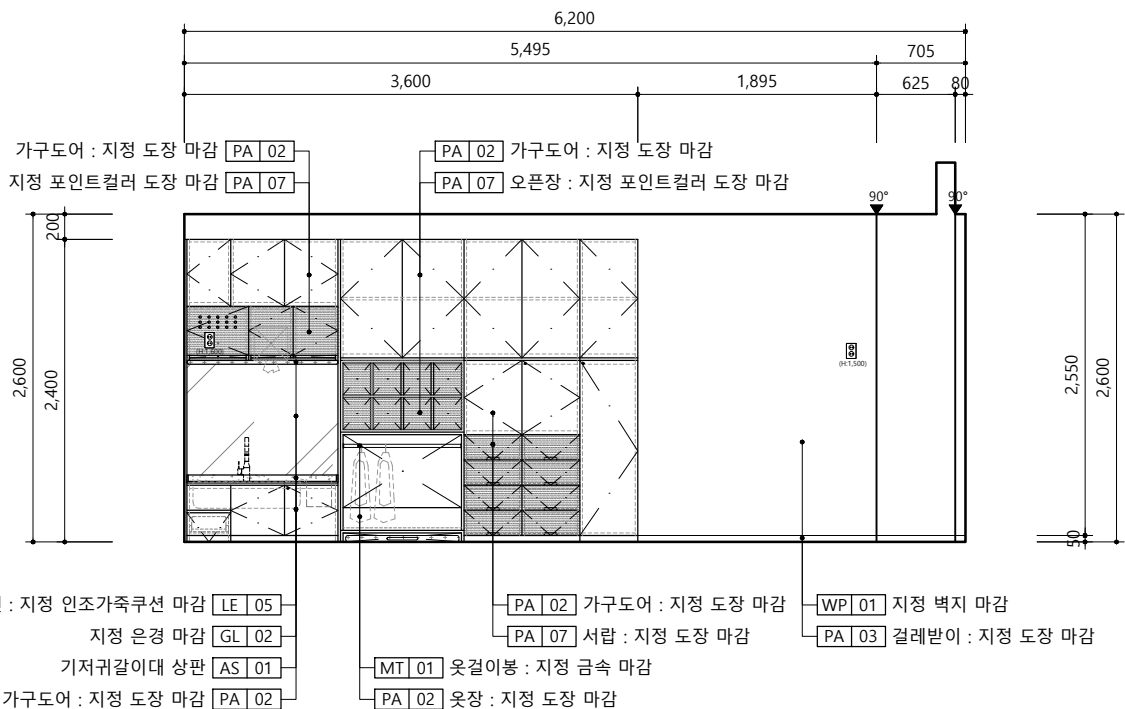
02 ELEVATION-B
