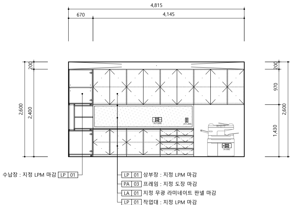
02 ELEVATION-B
